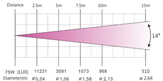
4. PHOTOMETRICS DIAGRAM
